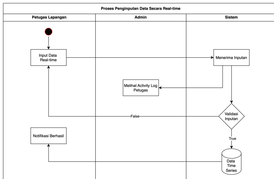
Gambar 3. 8 Activity Input Data Real-time
