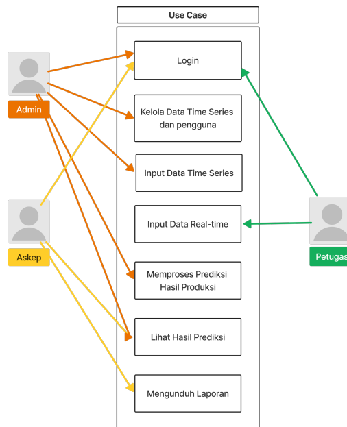
Gambar 3. 4 Use Case Diagram
